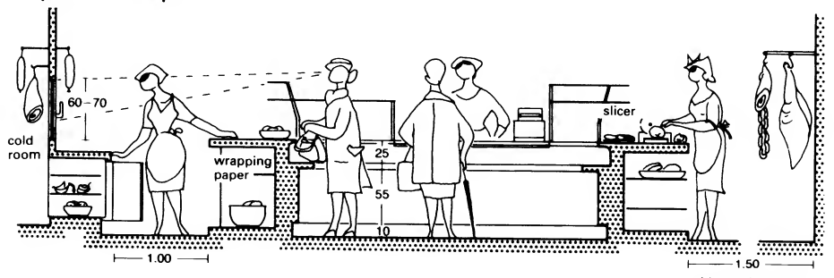
11 Normal butcher's counter (also for fishmonger's → 2)
